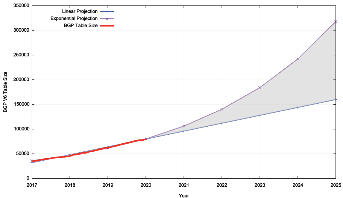
Figure 31 -Projections of IPv6 BGP Table Size
