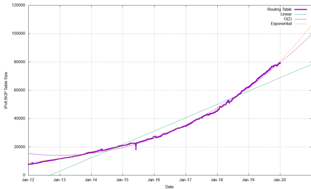
Figure 16 - IPv6 BGP Routing Table Size (RIB)
