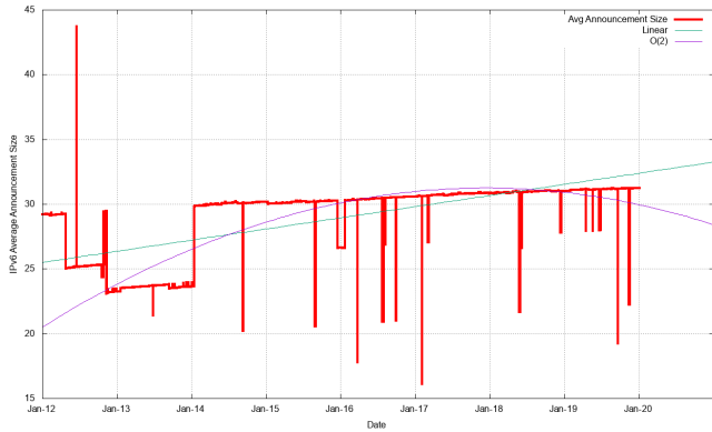
Figure 20 - IPv6 Average Prefix Size (Prefix Size)
