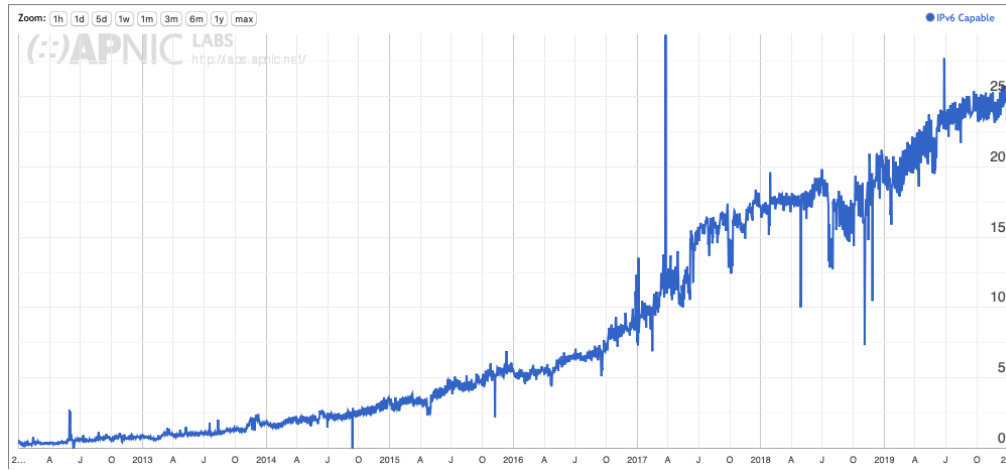
Figure 32 -IPv6 Deployment 2012 - 2020
