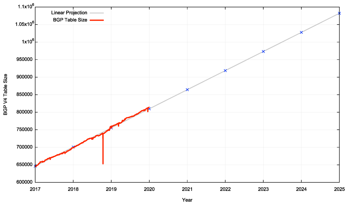
Figure 28 – Linear Prediction of IPv4 Table Growth
