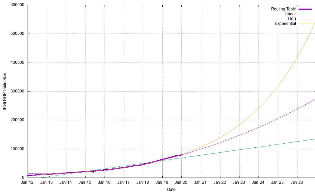
Figure 29 – IPv6 BGP Table Size from January 2012
