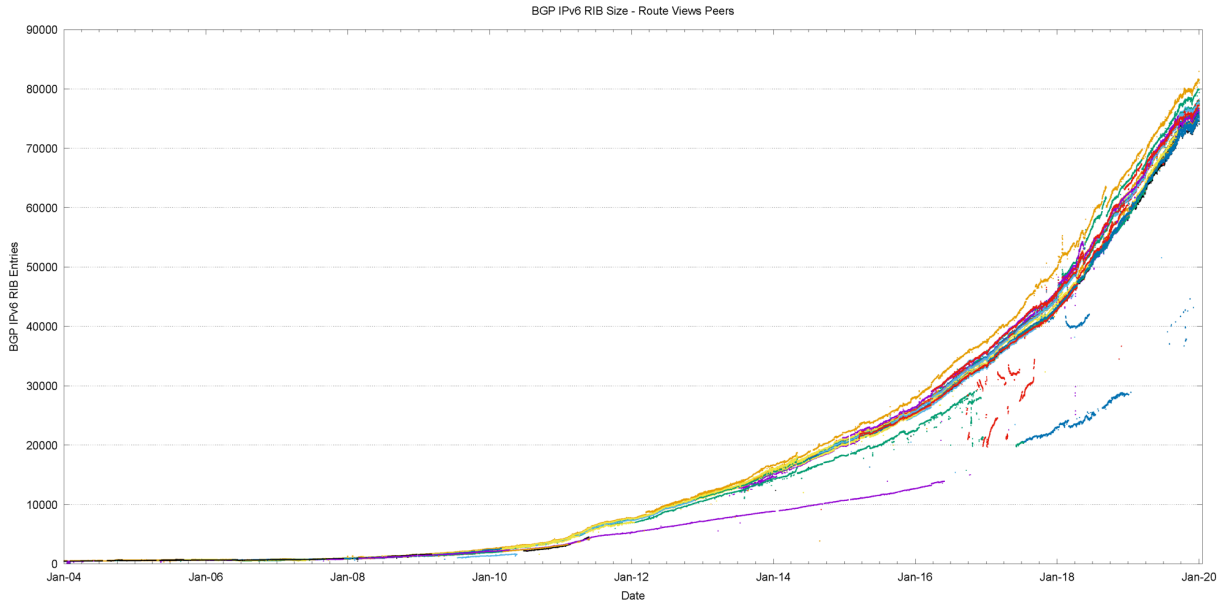
Figure 14 – IPv6 routing table since 2004 as seen by Route Views Peers
